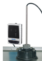
11452 - Overfill prevention complete, supply voltage 230 V, comprising: level sender
